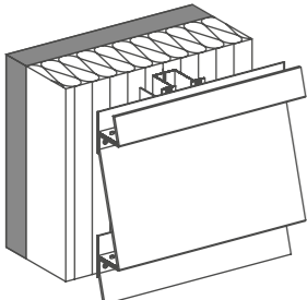
8 RIVETED WEATHER BOARDING on aluminium sub-construction
